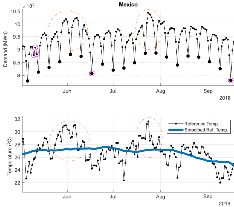
200 Fig. 4. Example of variations in the daily demand of Mexico due to the real demand, the magenta circles mark holidays. Bottom: Reference temperature (black) and smoothed reference temperature (blue).
