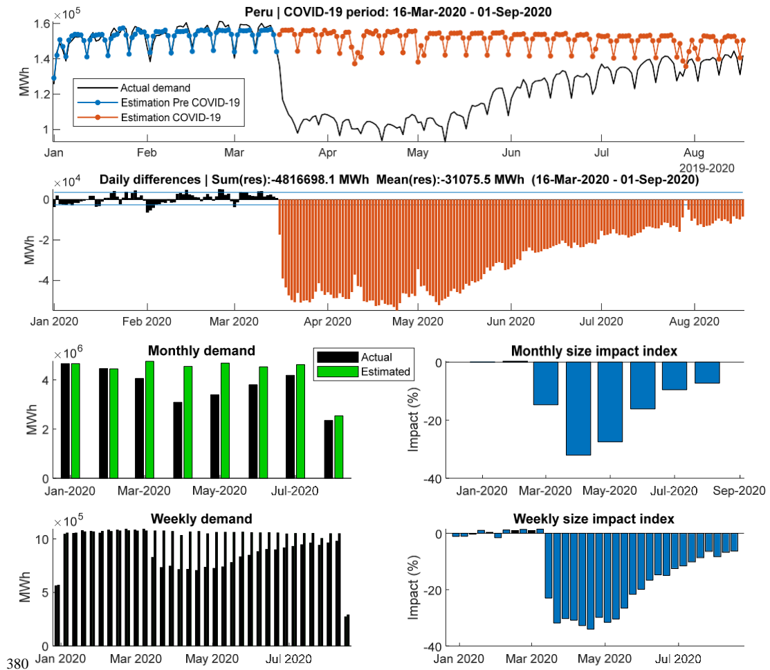
380 Fig. 10. Impact of COVID-19 on the demand in Peru during 2020. Thanks to the estimated reference demand, it can be stated that the demand suffered a very sharp decrease as of March 16th, 2020, reaching the maximum impact in the month of April, with an impact of -32%, the highest of all the countries studied. In August 2020, the demand had not yet recovered the 385 expected values according to the reference demand. Source: Extracted from [28] (Fig. 15, p. 23). © 2021 BID. Reprinted with permission of BID.
