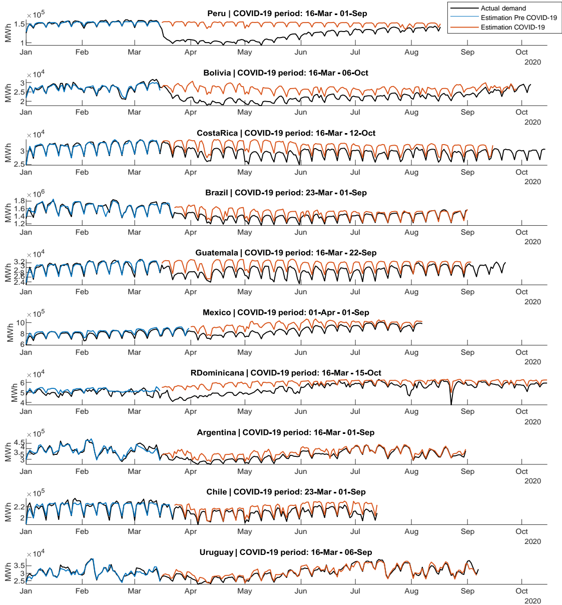
Fig. 14. Daily comparison for 2020 between the real demand (in black) and the reference demand estimated by the model. The reference demand is shown before the start of the effect of the pandemic (in blue) and during the pandemic (in orange).
