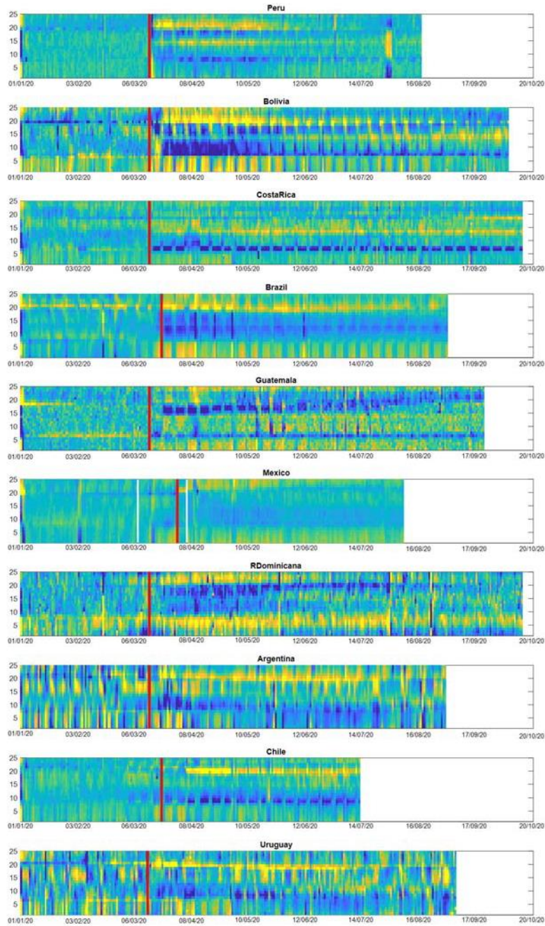
600 Fig. 18. Heat maps of the differences for each country during 2020. The vertical red line marks the start of confinement in each country.
