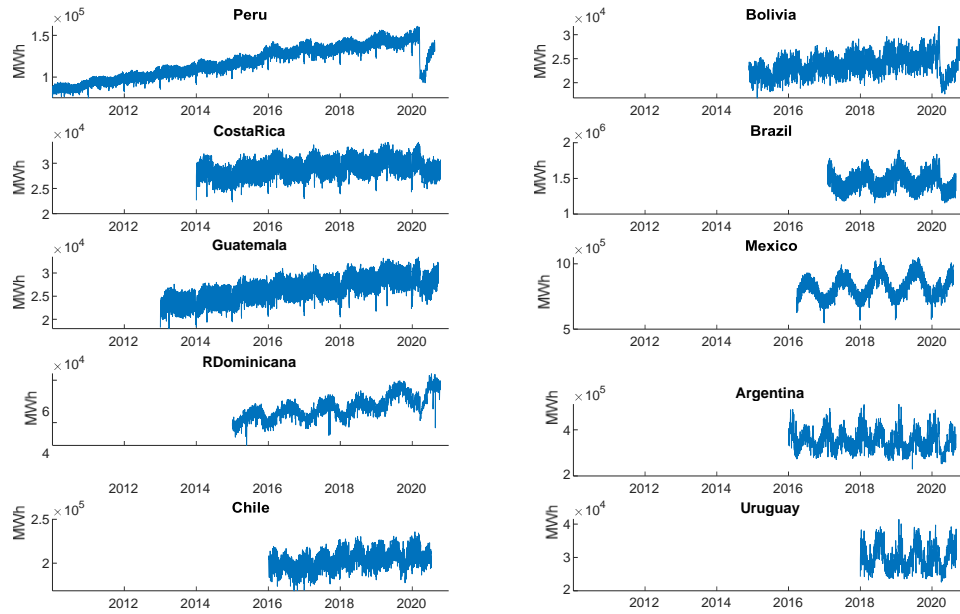
Fig. 2. Daily demand for the LAC countries.
