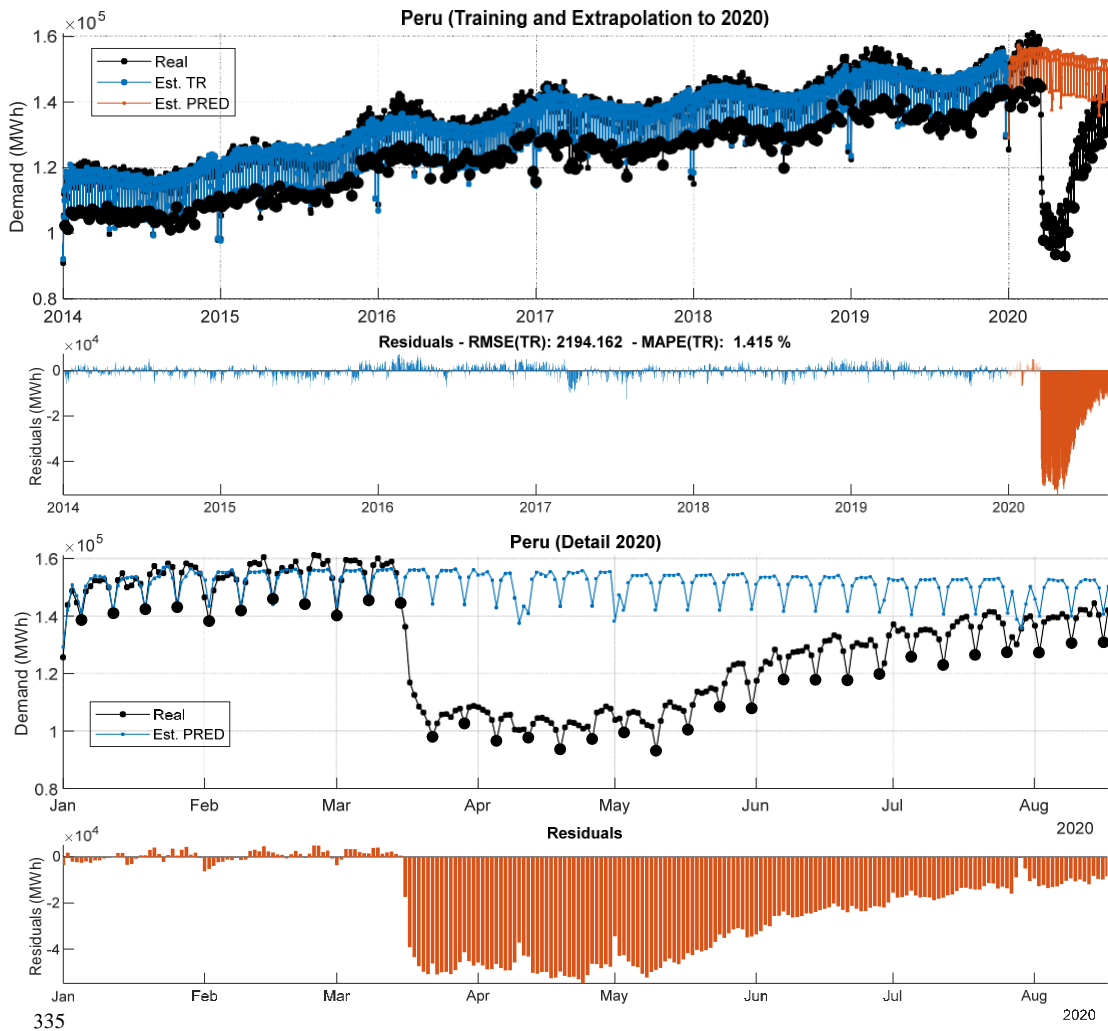
Fig. 9. Daily electricity demand for Peru.
